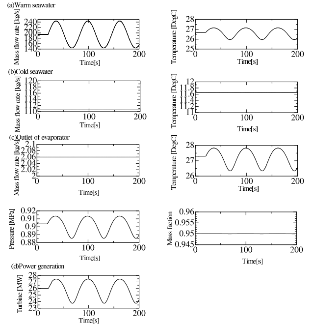
Fig. 8 Sine wave response result (OTEC part)
