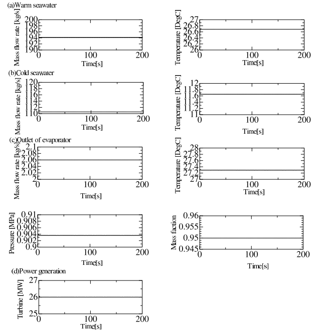
Fig. 4 Step response result (OTEC part)
