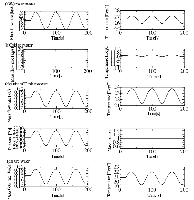
Fig. 9 Sine wave response result (Desalination part)
