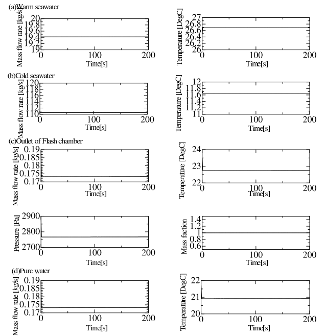
Fig. 5 Step response result (Desalination part)
