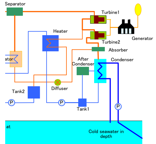
Fig. 1 OTEC system
