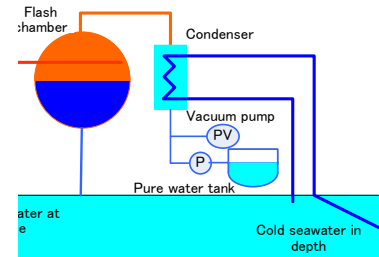
Fig. 2 Spray flash desalination system
